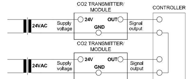
Figure 2 Connection of Separate AC Supplies (Recommended)
