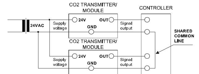
Figure 3 Connection of Single AC supply to Several Transmitters
