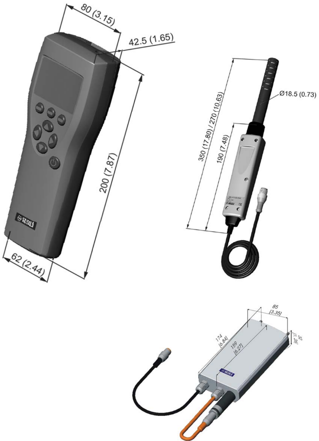
Figure 20 Dimensions
